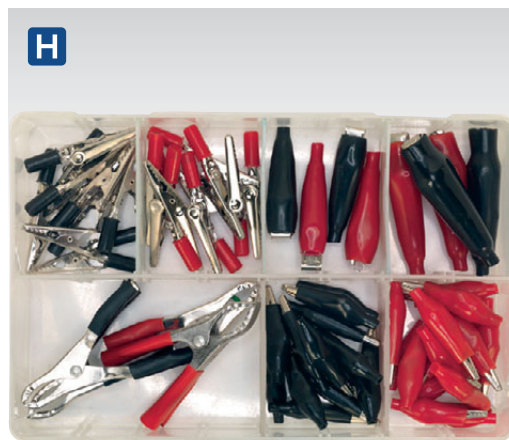
H H AB023CA 60pc Crocodile Clip Assortment Black & Red Contents (Approximate Quantity): Non-Insulated; 55 (x20), 70 (x2), 75mm (x2), Insulated; 45 (x16), 55 (x12), 60mm (x8)
