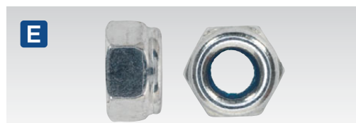
E SEE BELOW Zinc Plated Nylon Locknuts DIN 982 - M4-M16
