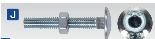
J SEE BELOW Zinc Plated Coach Bolt & Nuts DIN 603 - M6-M10
