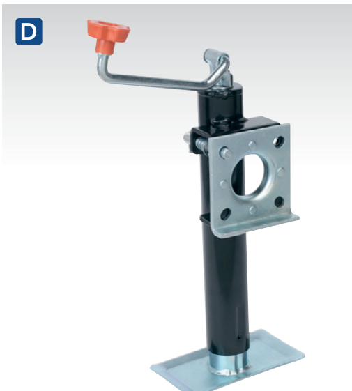
D TB373 Trailer Jack & Clamp 250mm Travel 900kg Capacity Heavy-duty trailer jack with swivel mounting. Suitable for handling trailers with heavy nose weight. Integral swivel weld-on mounting.
